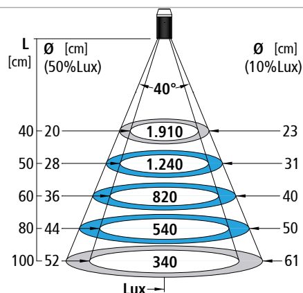
MN03 L40-F700-24ACDC
