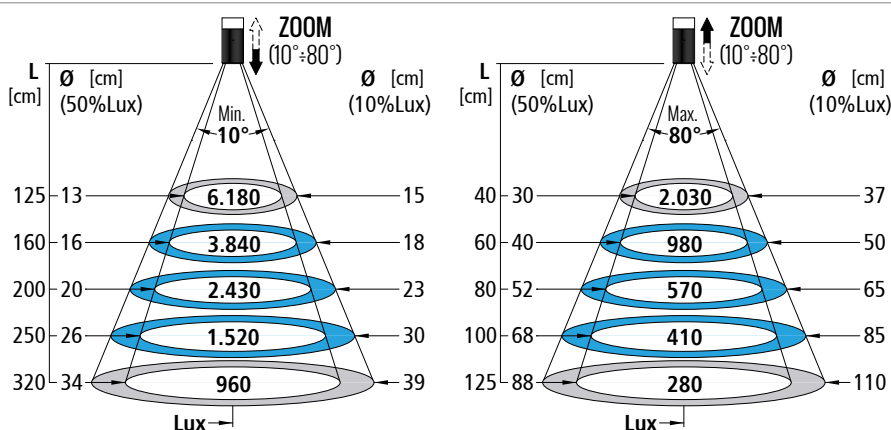
MN03 LZ-F700-24ACDC
