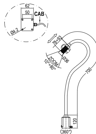
MN03 LZ-F700-100240AC
